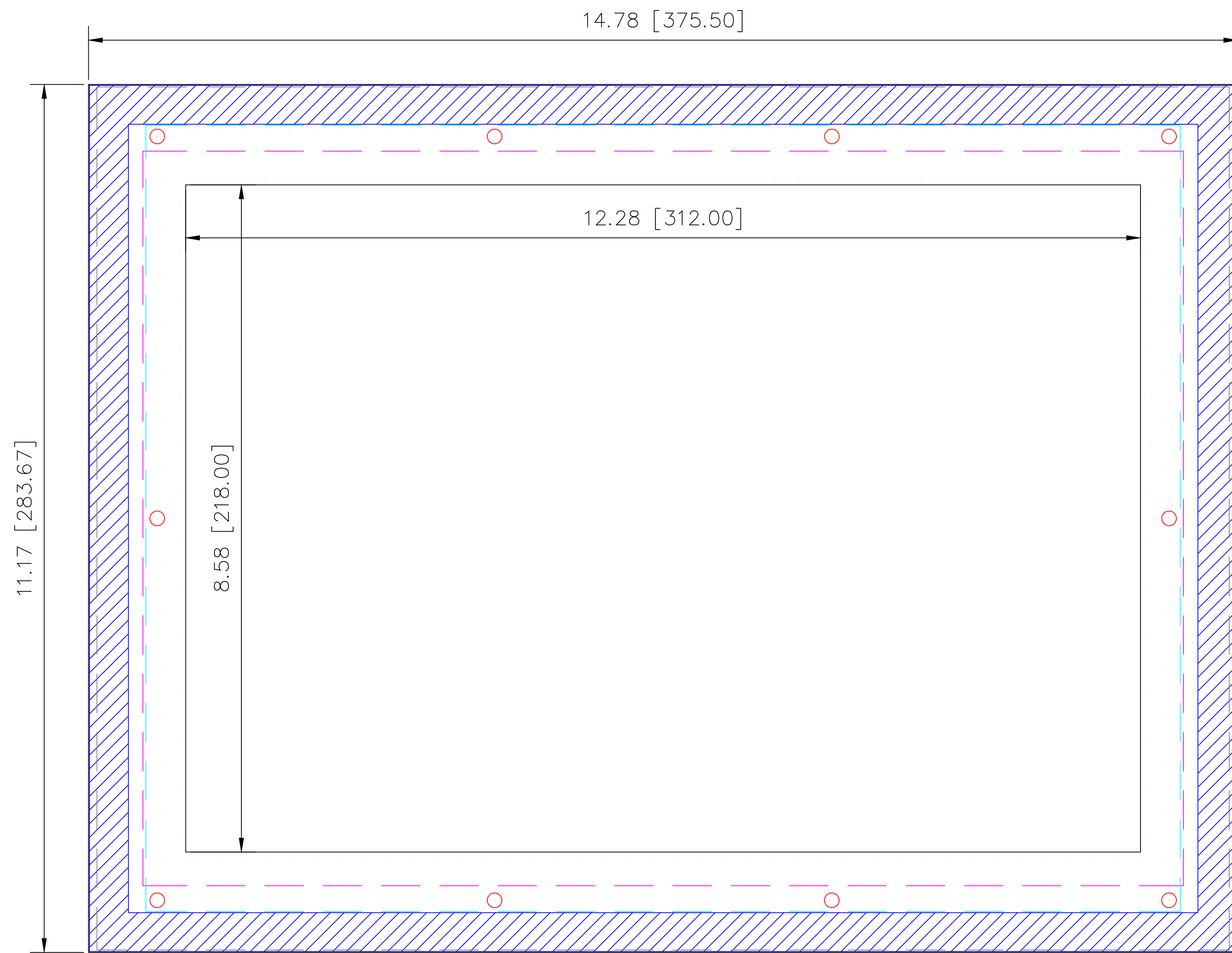
FRONTPLATE
