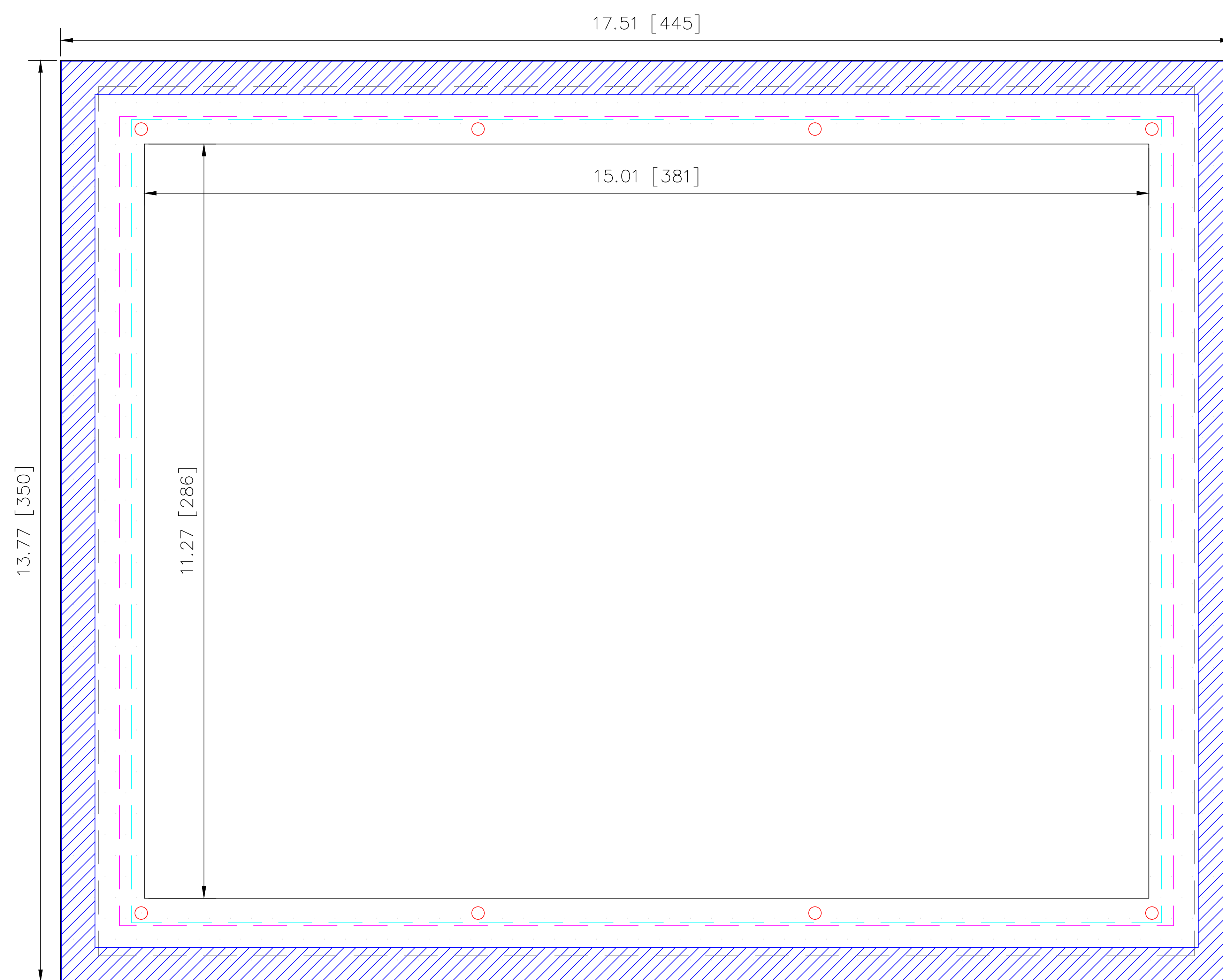
Front Plate
