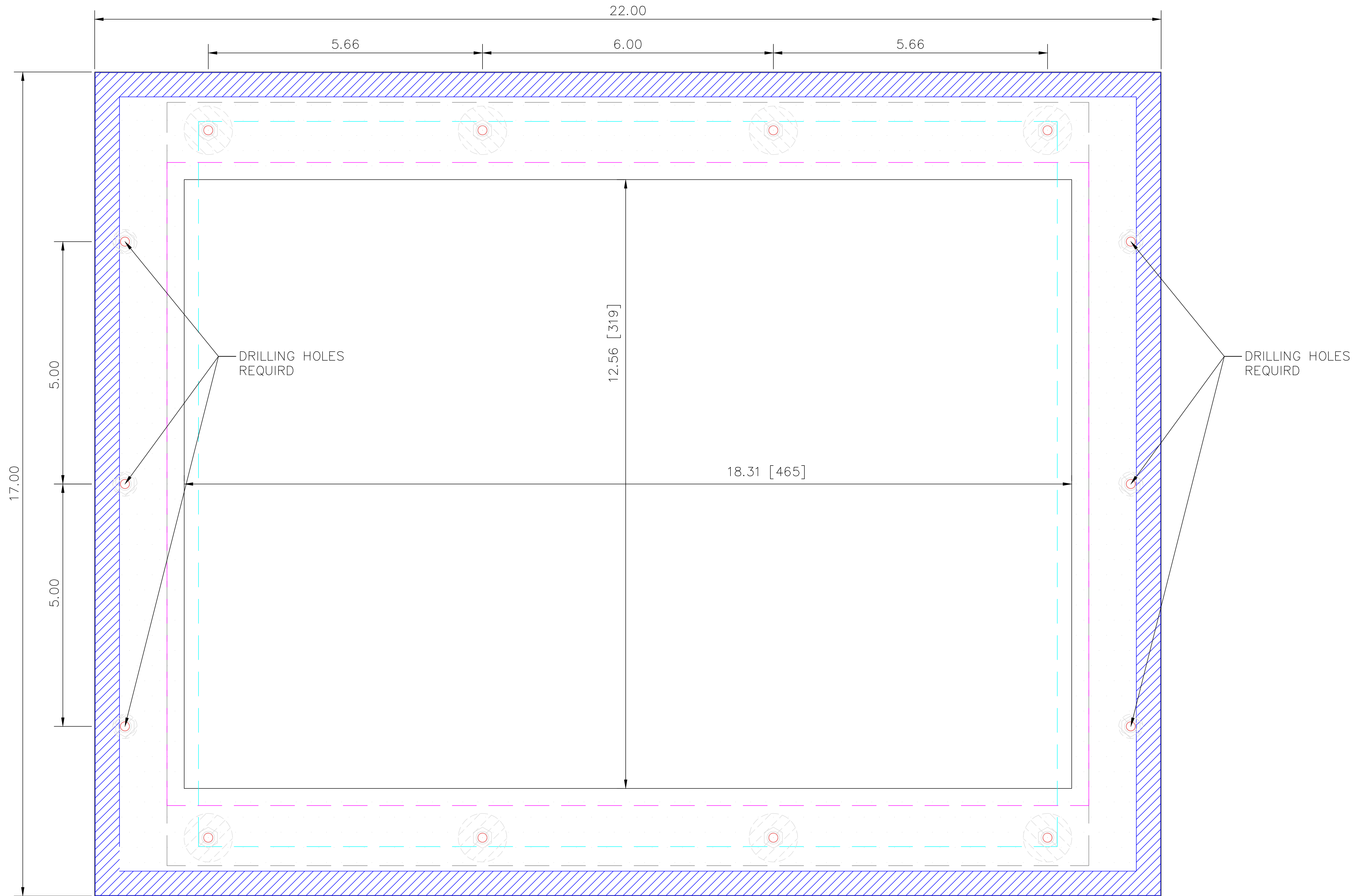
MODIFIED GENERATED DRAWING FOR STUD AND PLATE DIMENSIONS
